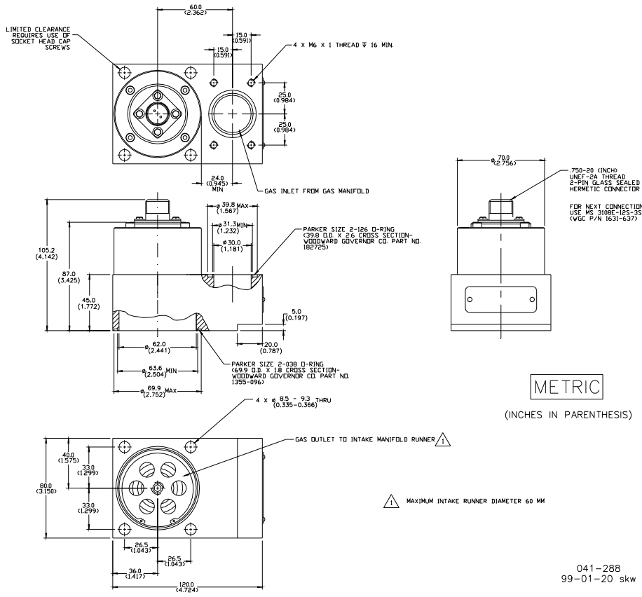
SOGAV 43 Outline Drawing (Do not use for construction)
